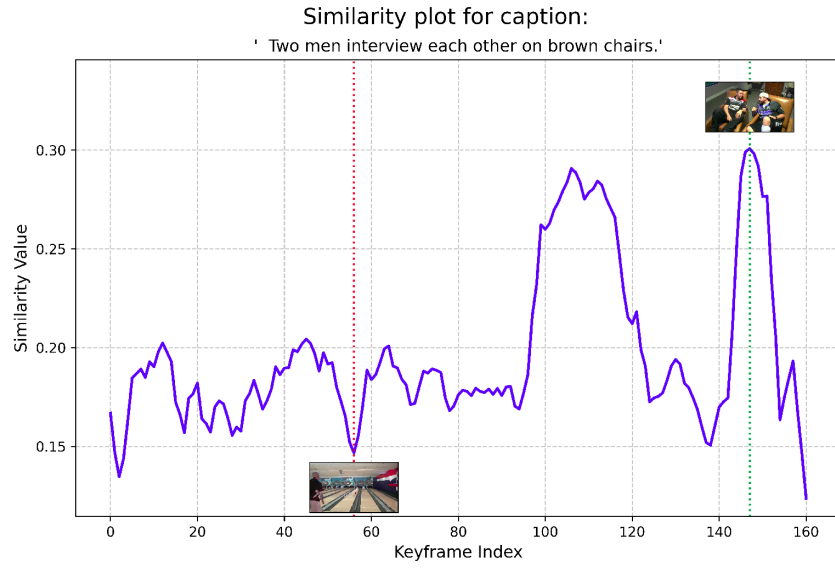
Fig. 9. Caption-Keyframe similarity score example 1
